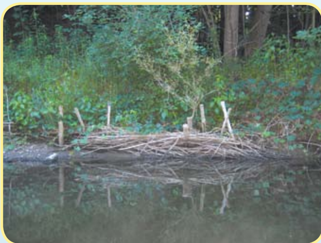
Figure 48 - Log matrix used to armor bank
