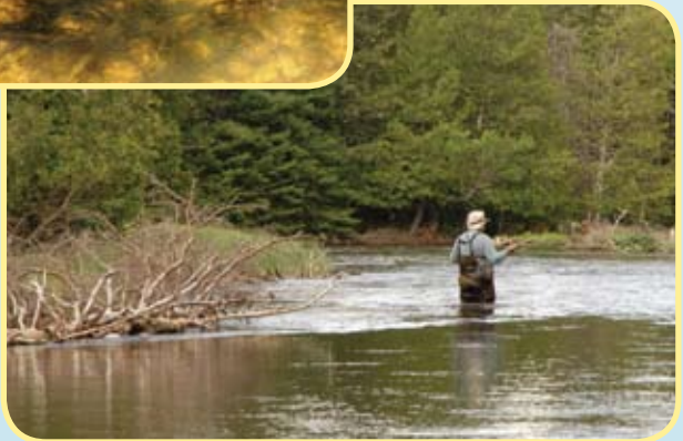
Figure 58 - LWD structures provide excellent habitat for a variety of game fish
